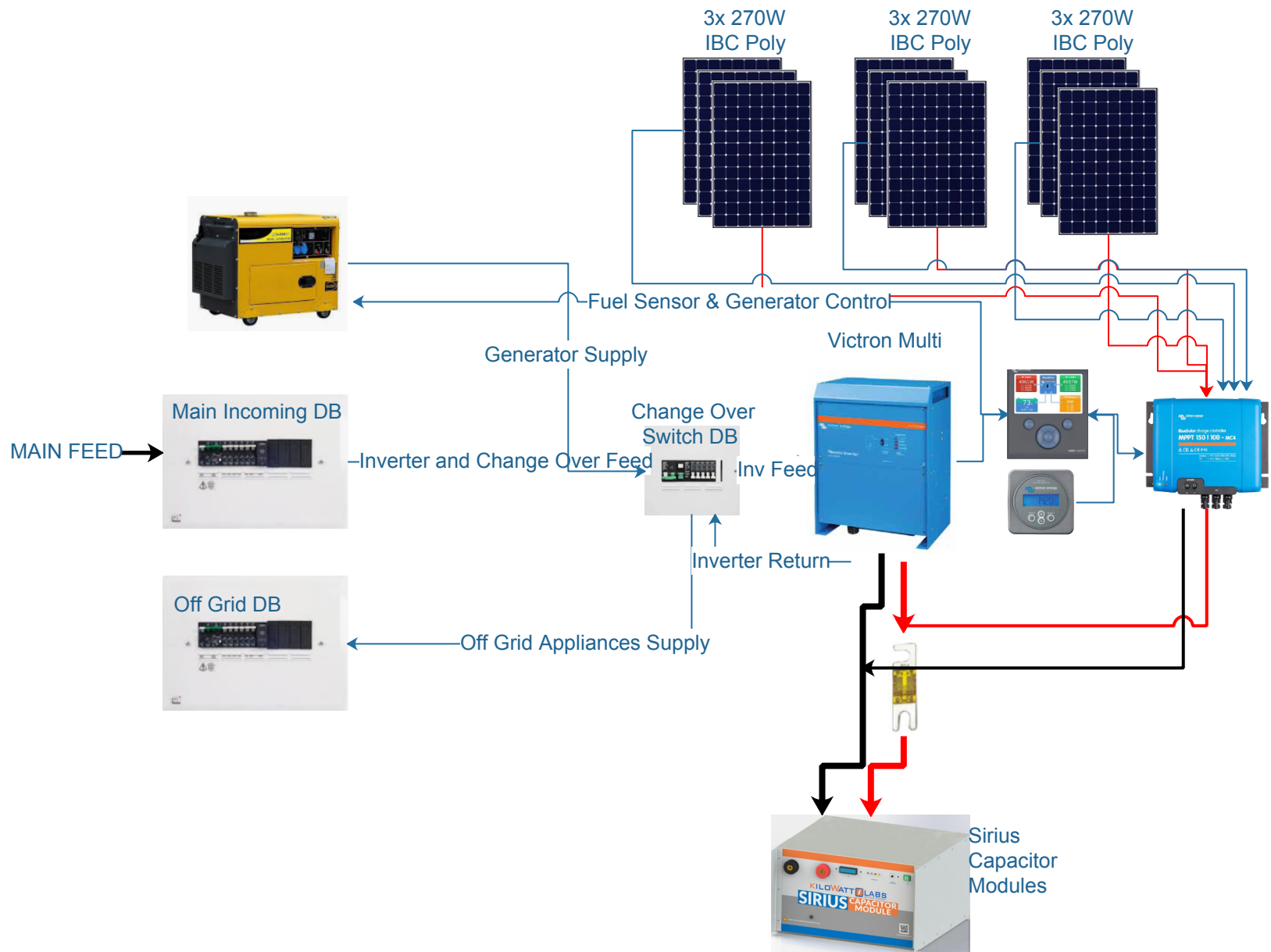
Off Grid Schematic Layout
